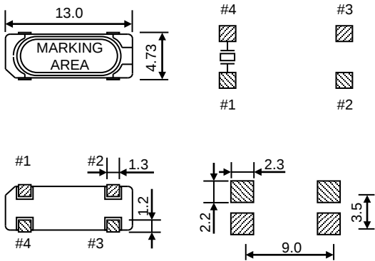
HC-49SN
