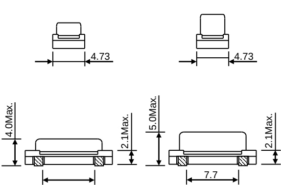
HC-49SNC
